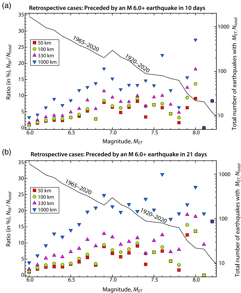
Figure 2. Historical retrospective occurrence percentage for an earthquake (mainshock) with the given magnitude preceded by an M \geq 6.0 event (foreshock) within different radial distances (50–1000 km) over time ranges of (a) 10 days and (b) 21 days. Colored symbols indicate the occurrence percentage for foreshock–mainshock pairs (left scale) found for different search distances. Other symbols are the same as Figure 1. The color version of this figure is available only in the electronic edition.
