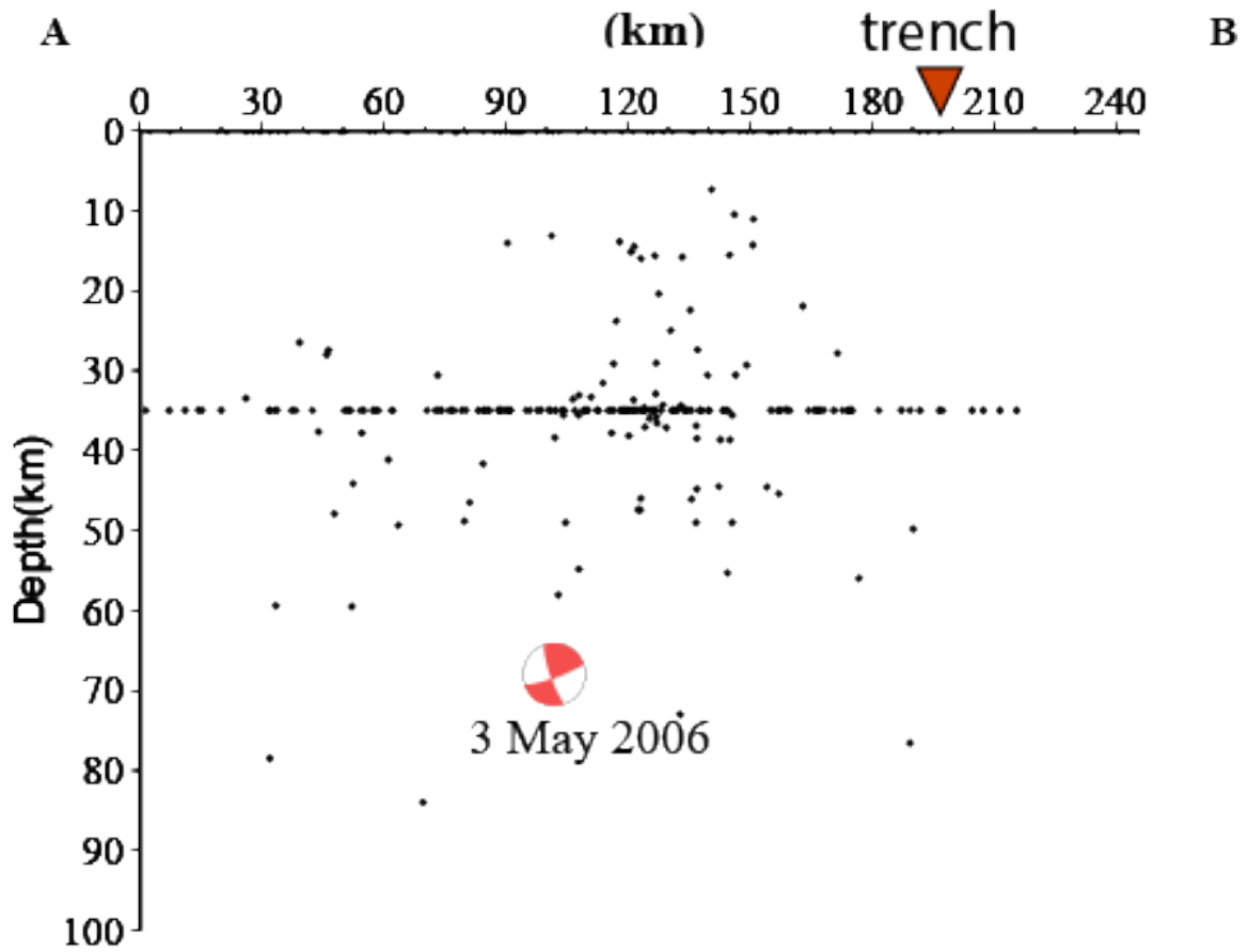
Figure S1. Cross-section view of aftershocks from the USGS-NEIC catalog for the 3 May 2006 Tonga event along profile AB in Figure 2. The scatter in the catalog locations is too large to confidently identify the megathrust, but the mainshock hypocenter clearly plots below the distributed aftershocks.
