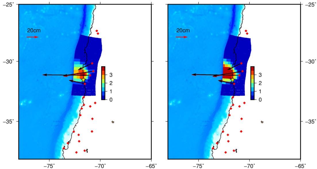
Figure 13. Slip inversions based on co-seismic displacements from GPS (left) and GPS/GLONASS (right) using a curved fault with 330 individual patches. The red vectors denote observed co-seismic static offsets, and the black ones represent synthetic values.
